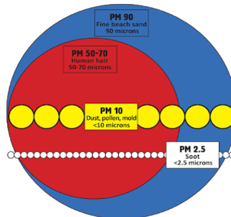
Small Particles found in smoke (PM10 and PM2.5) are smaller than a human hair.
